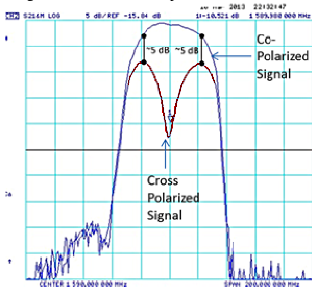
Figure 1 - Response of a Single Feed Antenna versus Response of an Accutenna antenna
